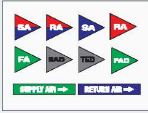
Duct Marking Labels (DW 144, BS 1710, ASME/ANSI)
